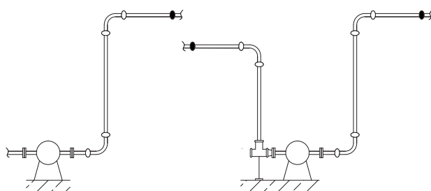
● Rigid coupling
