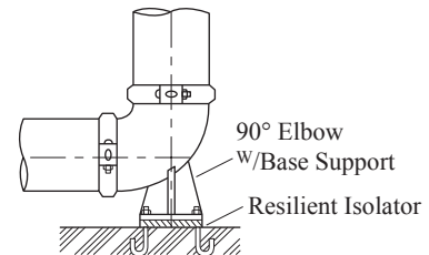
Anchor ( ->-> )
